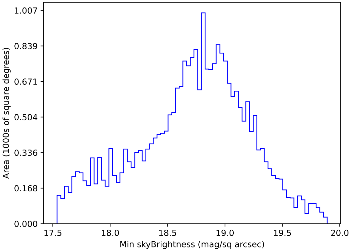
no_high_blob_v3.3_10yrs Yr 1 i band: Min skyBrightness
