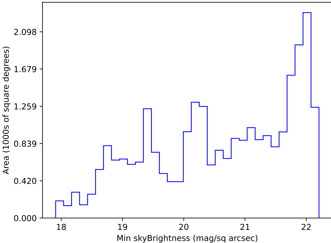
no_high_blob_v3.3_10yrs Yr 1 g band: Min skyBrightness
