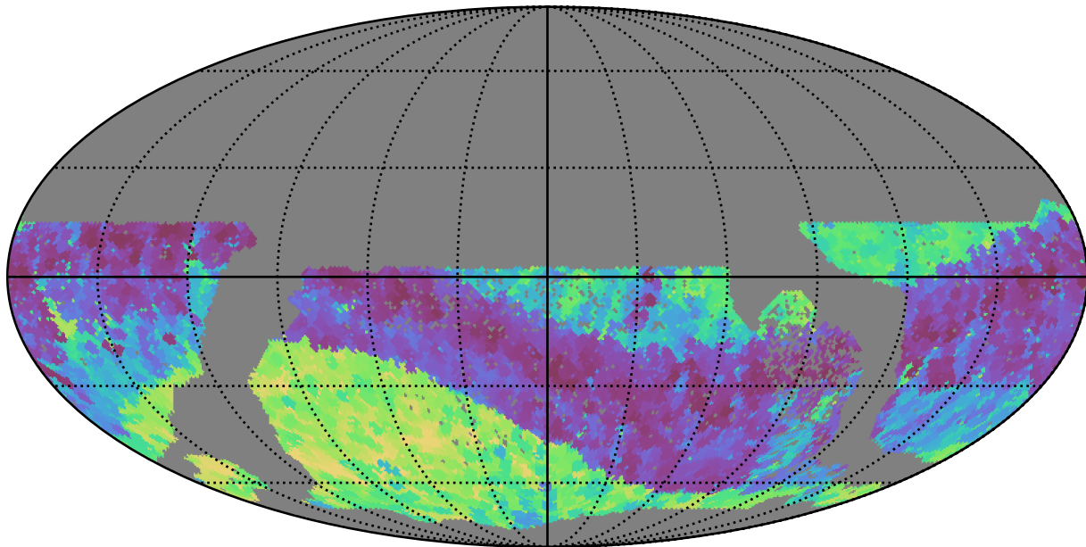
no_high_blob_v3.3_10yrs WFD z band: Min skyBrightness
