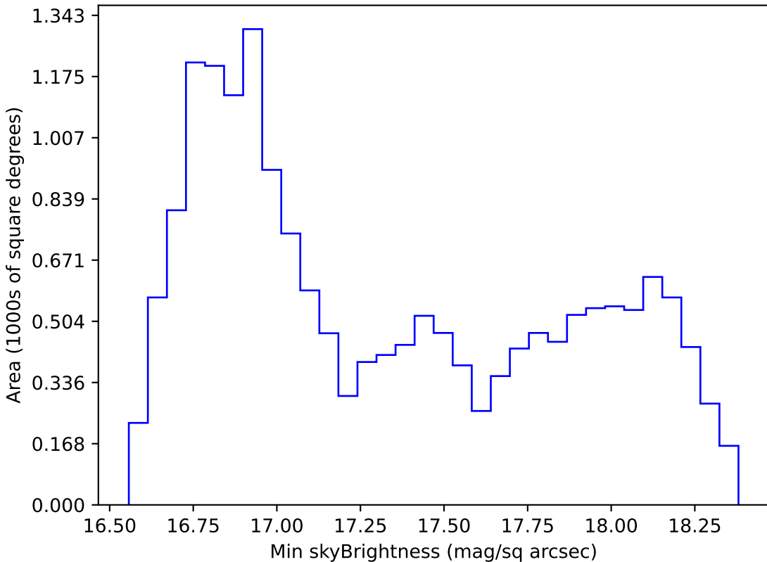
no_high_blob_v3.3_10yrs WFD z band: Min skyBrightness
