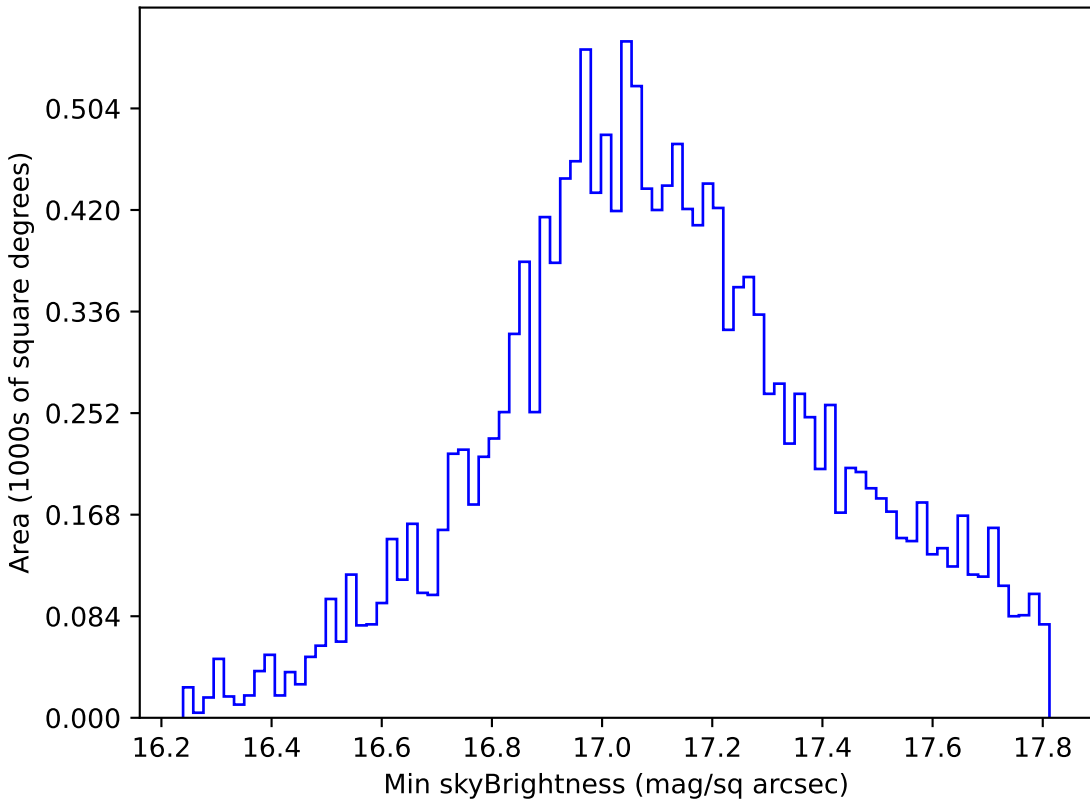
no_high_blob_v3.3_10yrs WFD y band: Min skyBrightness
