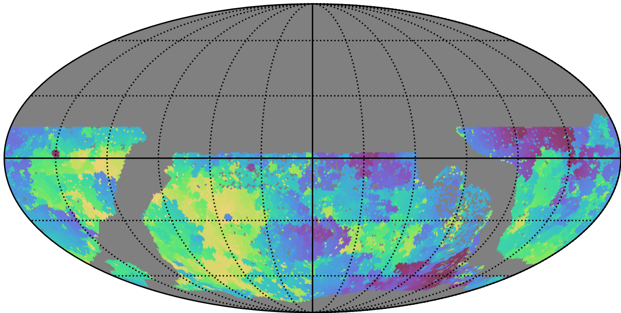
no_high_blob_v3.3_10yrs WFD u band: Min skyBrightness
