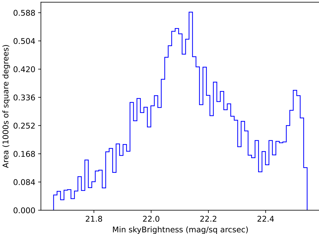
no_high_blob_v3.3_10yrs WFD u band: Min skyBrightness
