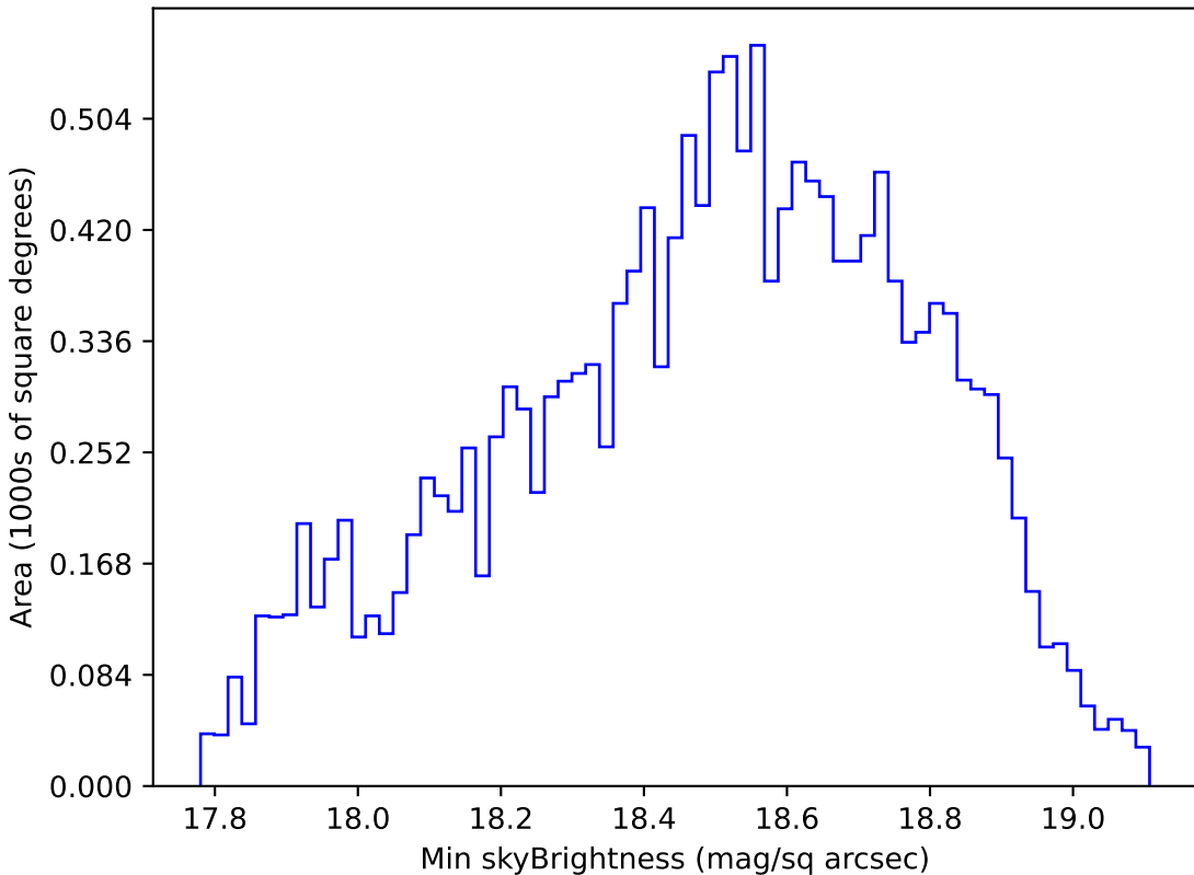
no_high_blob_v3.3_10yrs WFD r band: Min skyBrightness
