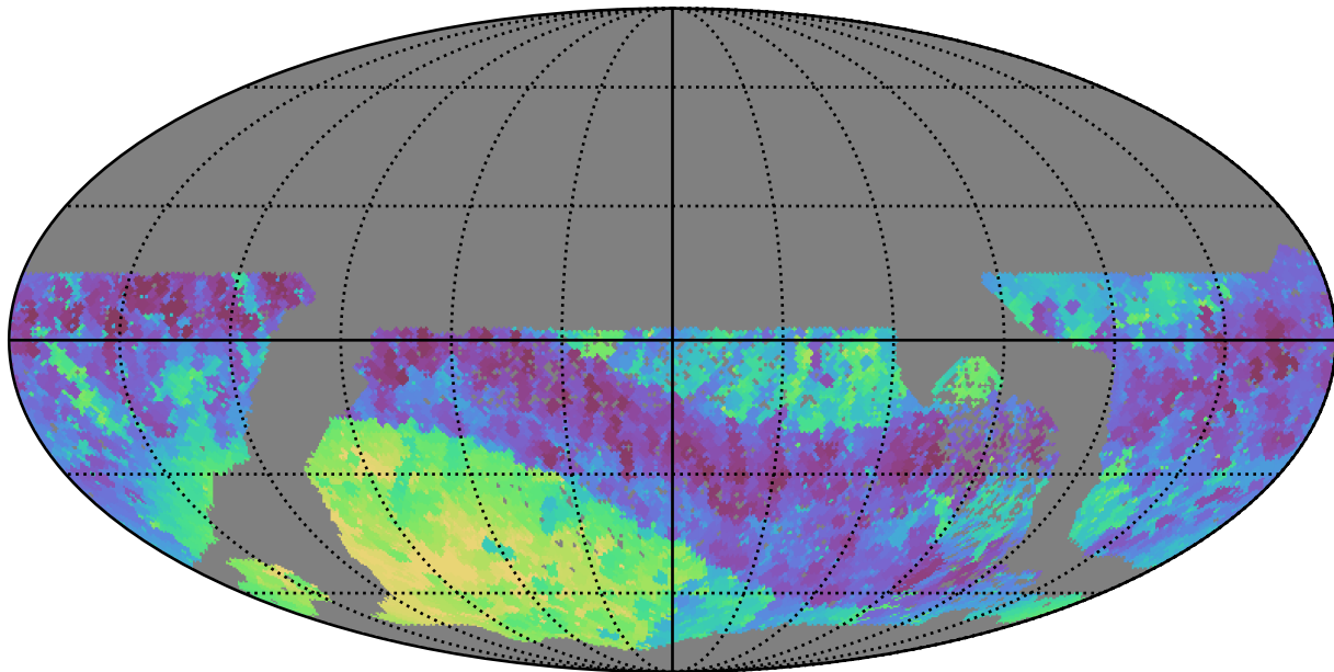
no_high_blob_v3.3_10yrs WFD i band: Min skyBrightness
