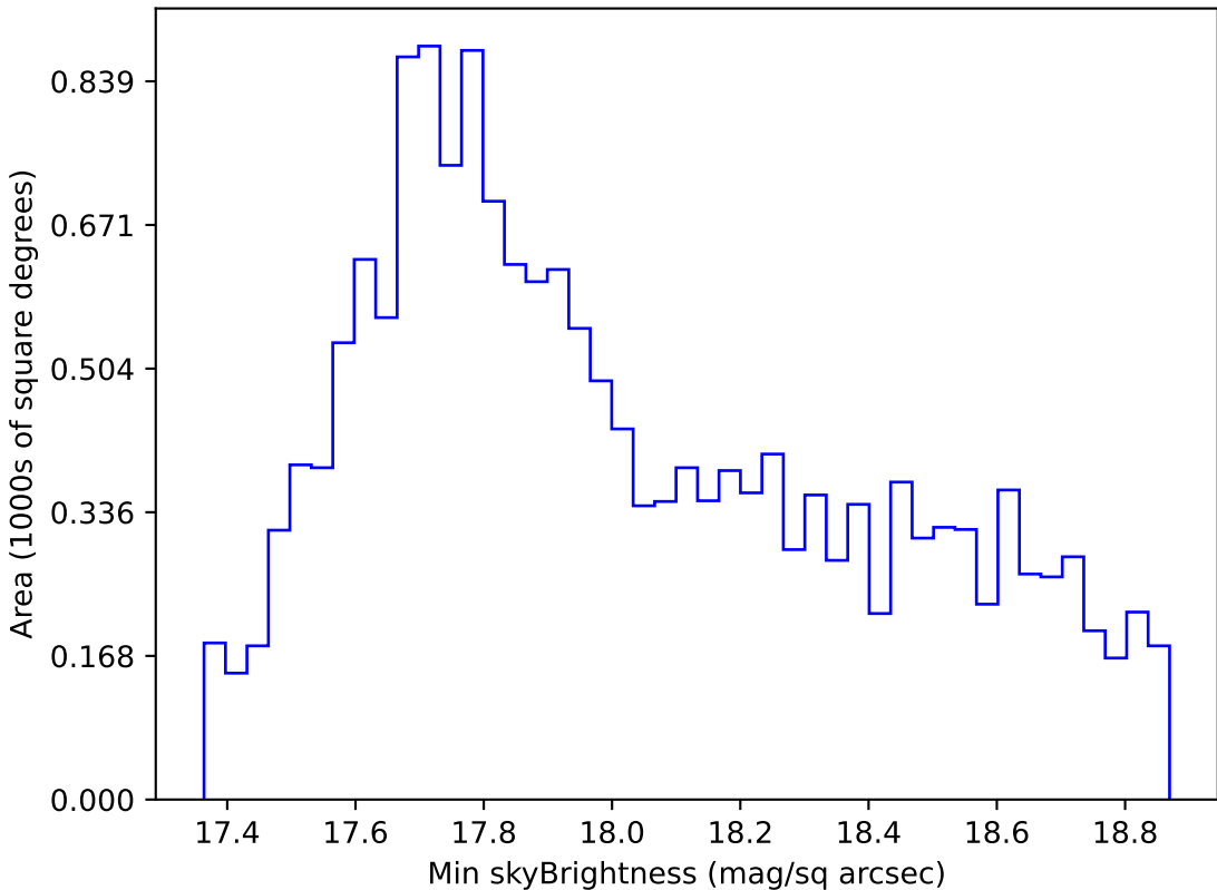
no_high_blob_v3.3_10yrs WFD i band: Min skyBrightness
