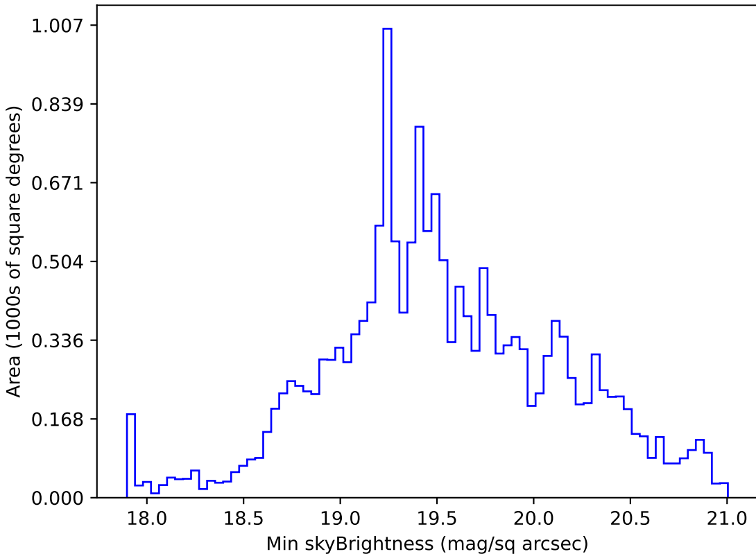
no_high_blob_v3.3_10yrs WFD g band: Min skyBrightness
