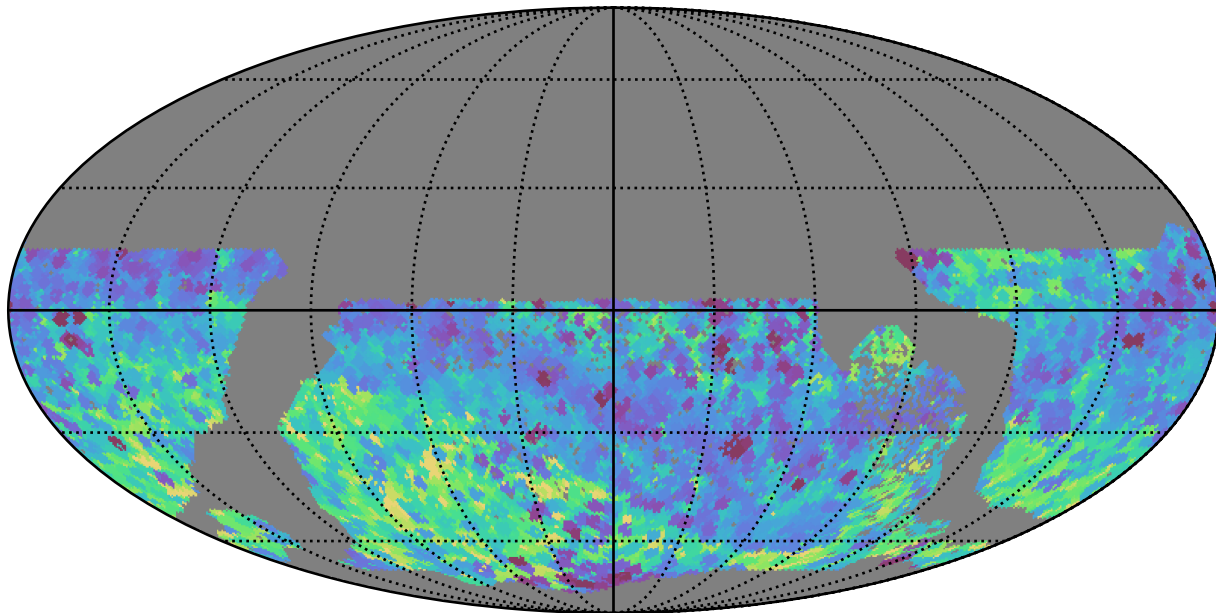
no_high_blob_v3.3_10yrs WFD all bands: Min skyBrightness
