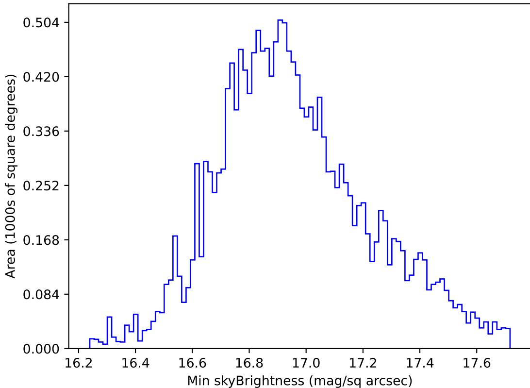
no_high_blob_v3.3_10yrs WFD all bands: Min skyBrightness
