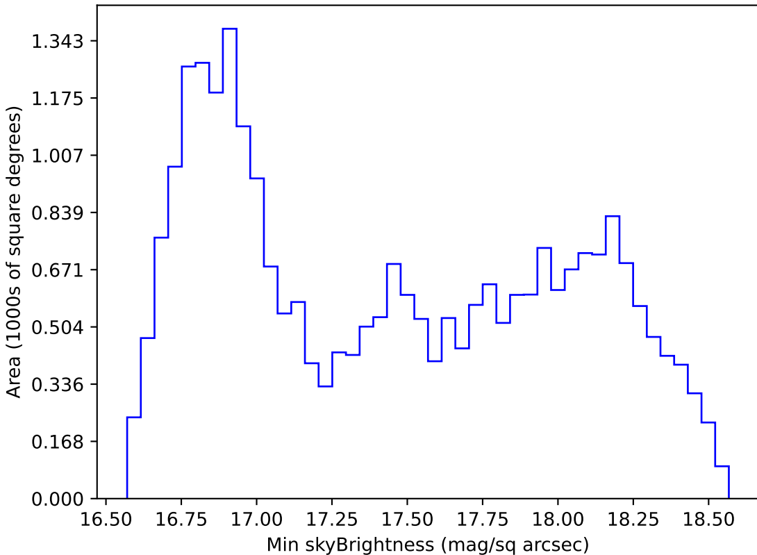
no_high_blob_v3.3_10yrs All sky z band: Min skyBrightness
