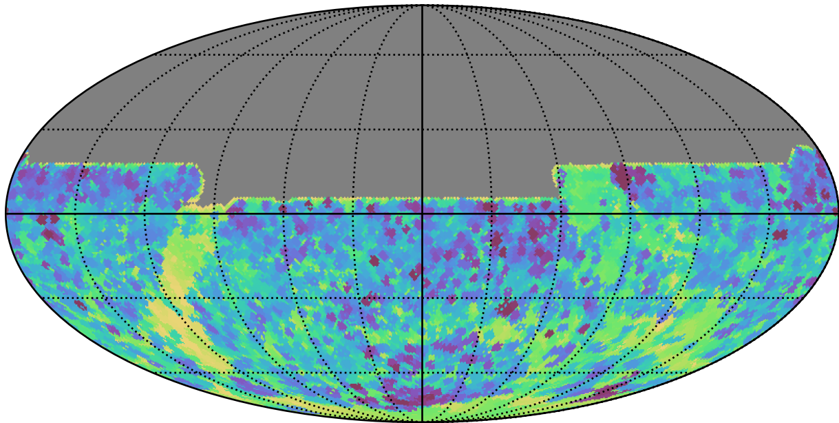
no_high_blob_v3.3_10yrs All sky y band: Min skyBrightness
