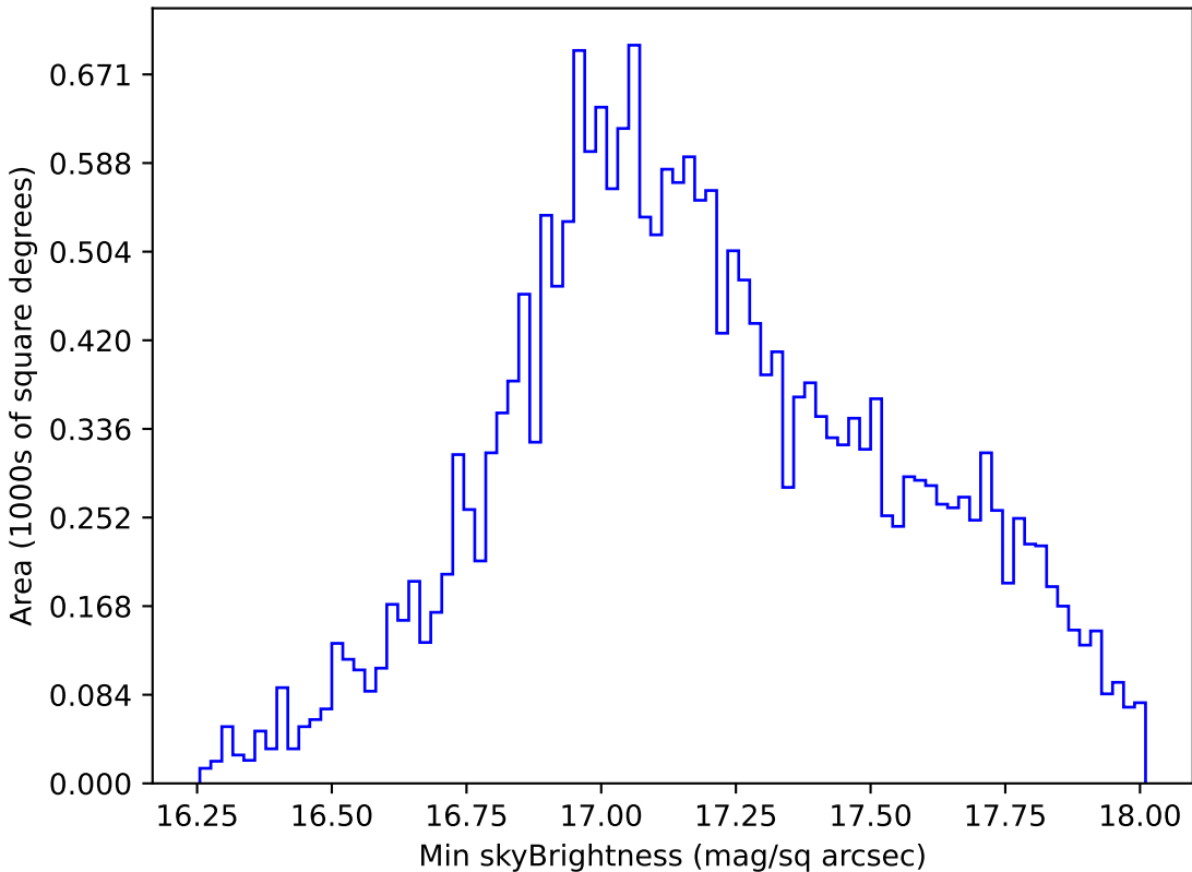
no_high_blob_v3.3_10yrs All sky y band: Min skyBrightness
