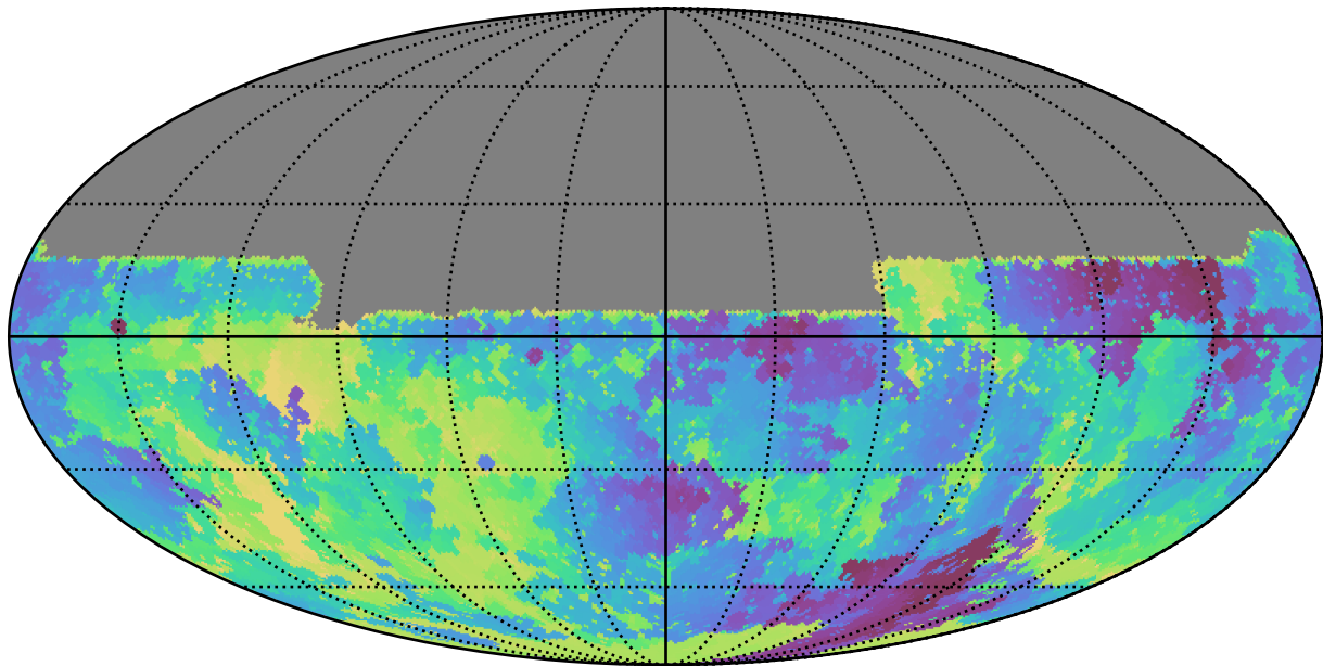
no_high_blob_v3.3_10yrs All sky u band: Min skyBrightness
