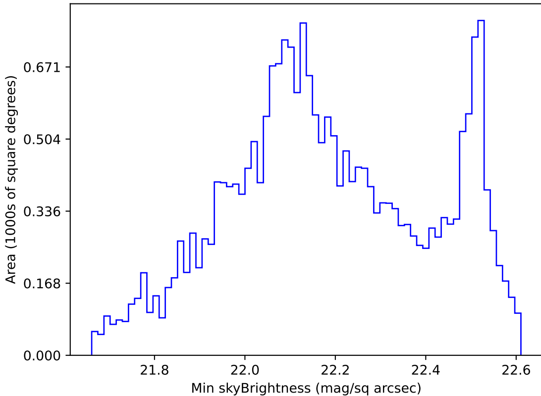
no_high_blob_v3.3_10yrs All sky u band: Min skyBrightness
