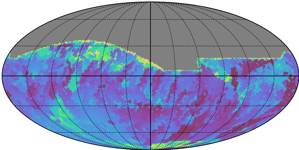
no_high_blob_v3.3_10yrs All sky r band: Min skyBrightness
