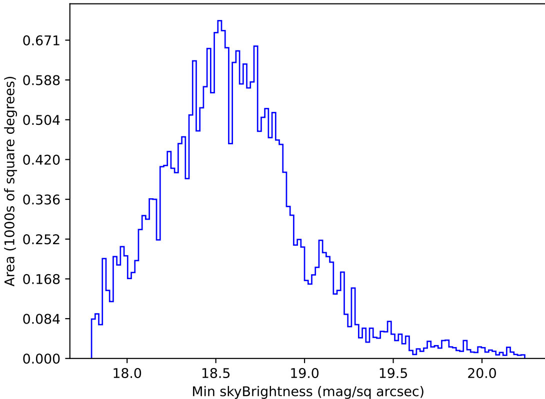
no_high_blob_v3.3_10yrs All sky r band: Min skyBrightness
