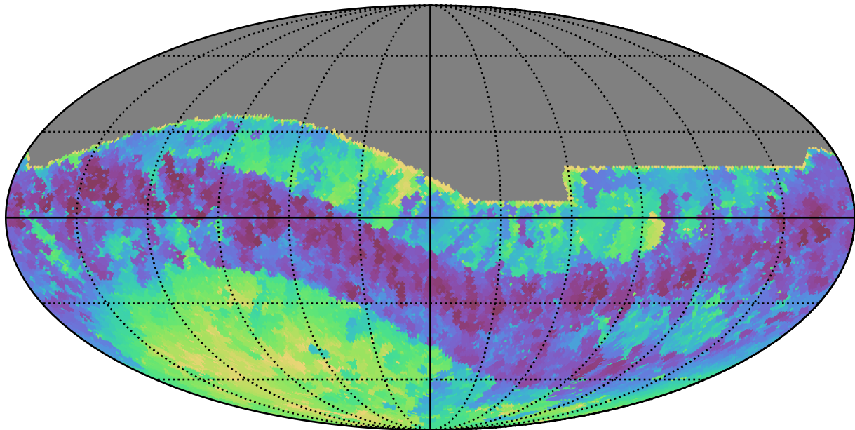
no_high_blob_v3.3_10yrs All sky i band: Min skyBrightness
