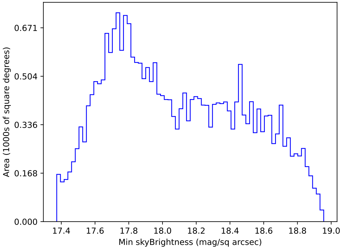
no_high_blob_v3.3_10yrs All sky i band: Min skyBrightness
