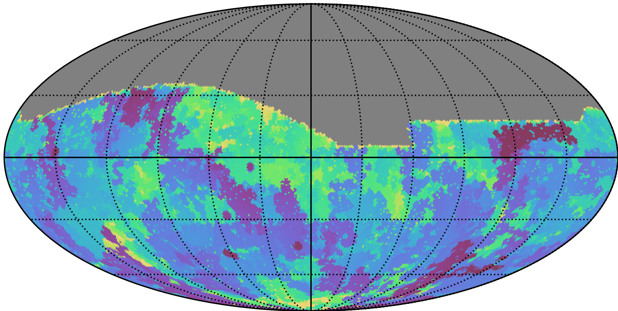
no_high_blob_v3.3_10yrs All sky g band: Min skyBrightness
