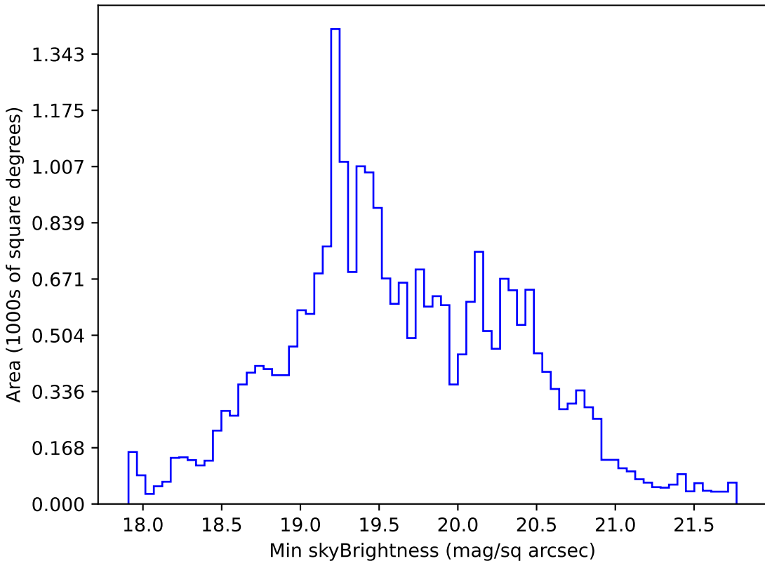
no_high_blob_v3.3_10yrs All sky g band: Min skyBrightness
