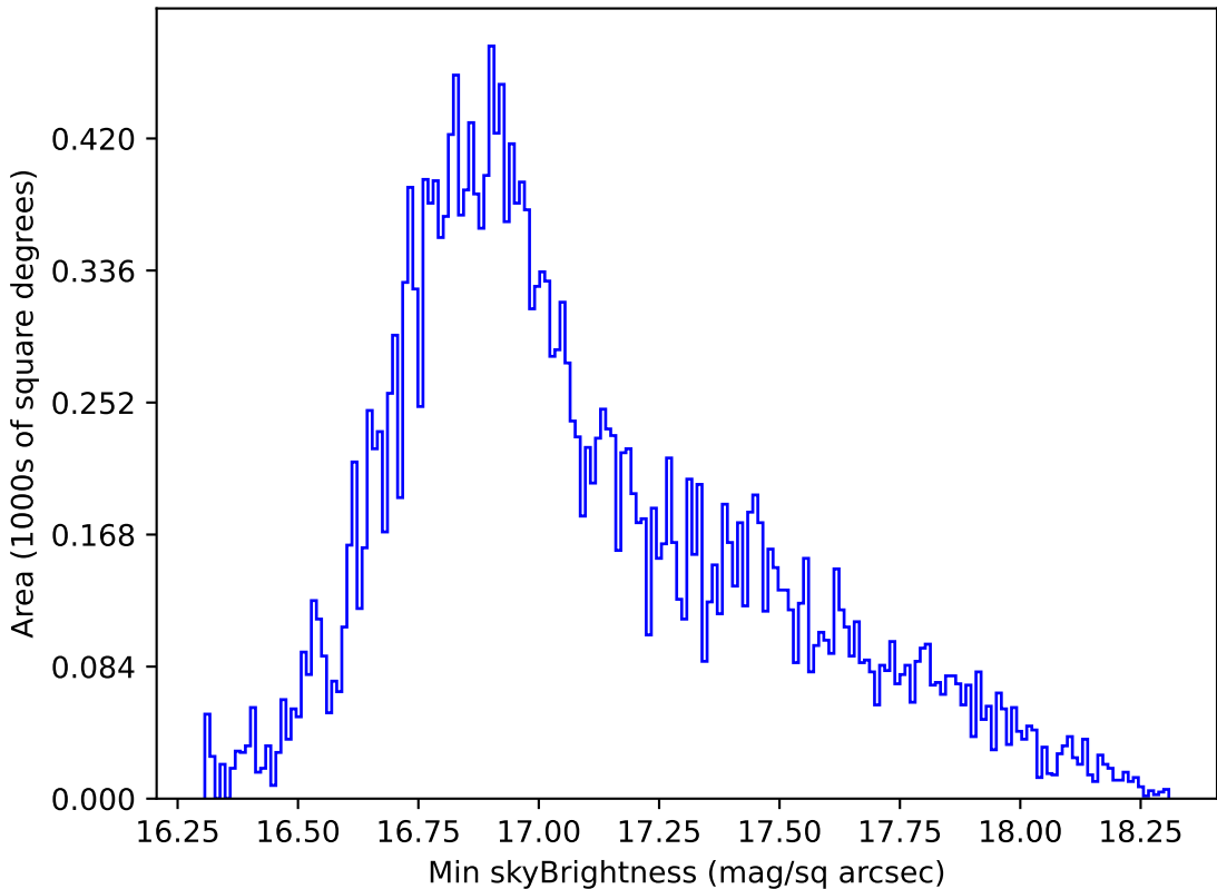
no_high_blob_v3.3_10yrs All sky all bands: Min skyBrightness
