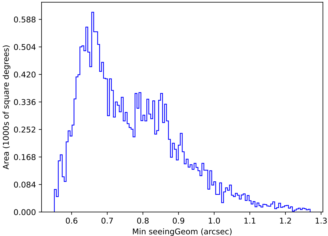
no_high_blob_v3.3_10yrs Yr 1 u band: Min seeingGeom
