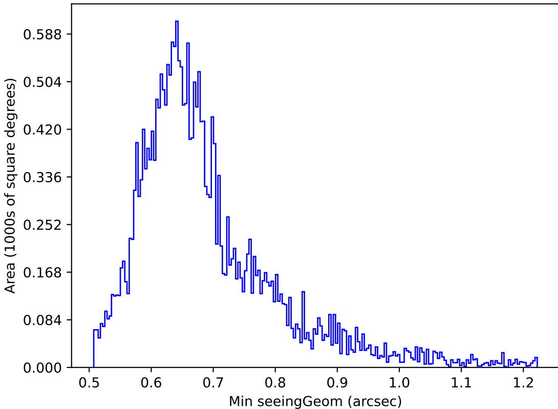
no_high_blob_v3.3_10yrs Yr 1 g band: Min seeingGeom
