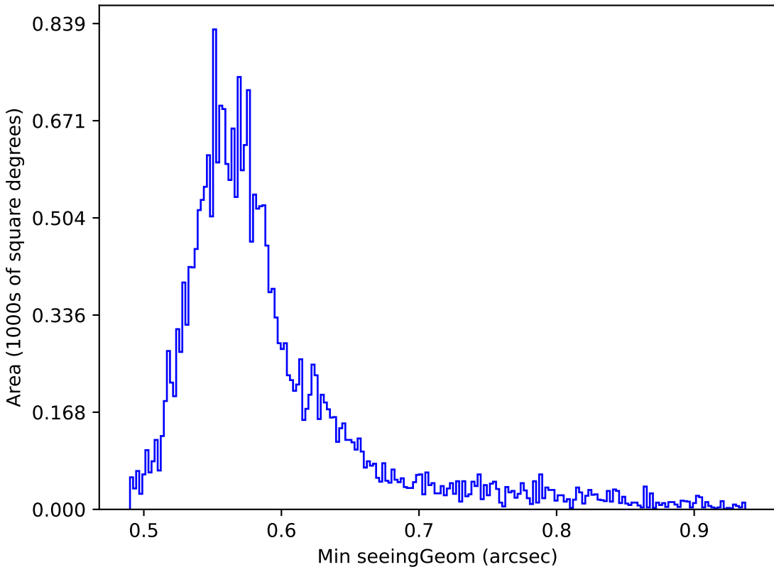
no_high_blob_v3.3_10yrs Yr 1 all bands: Min seeingGeom
