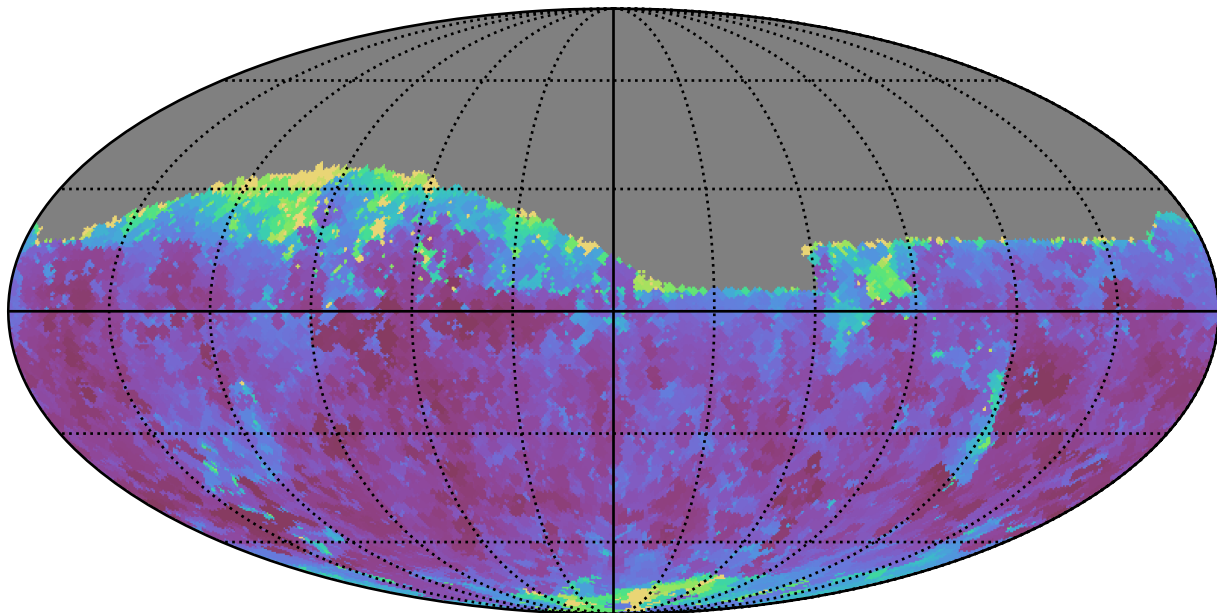
no_high_blob_v3.3_10yrs Yr 1 z band: Min seeingEff
