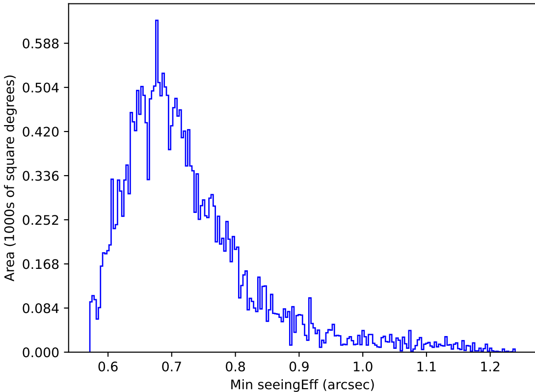
no_high_blob_v3.3_10yrs Yr 1 z band: Min seeingEff
