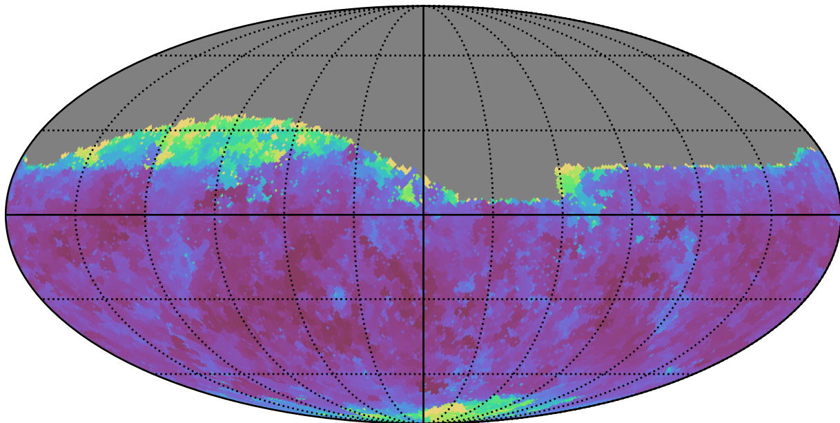
no_high_blob_v3.3_10yrs Yr 1 r band: Min seeingEff
