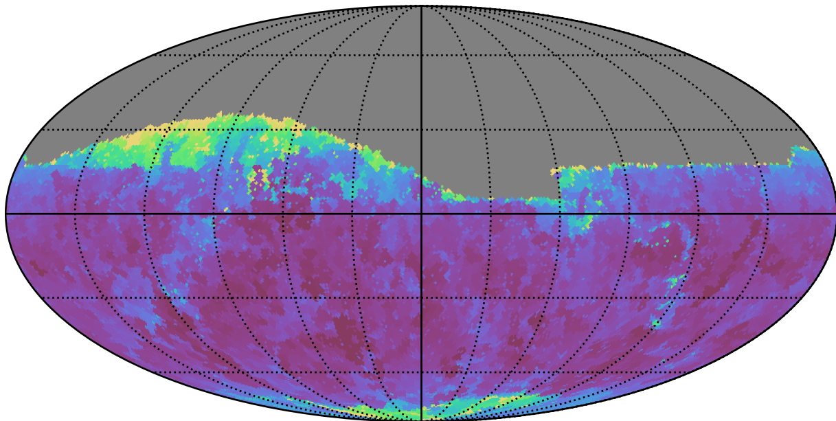
no_high_blob_v3.3_10yrs Yr 1 i band: Min seeingEff
