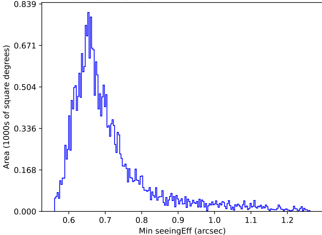
no_high_blob_v3.3_10yrs Yr 1 i band: Min seeingEff
