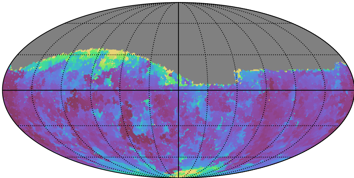
no_high_blob_v3.3_10yrs Yr 1 g band: Min seeingEff
