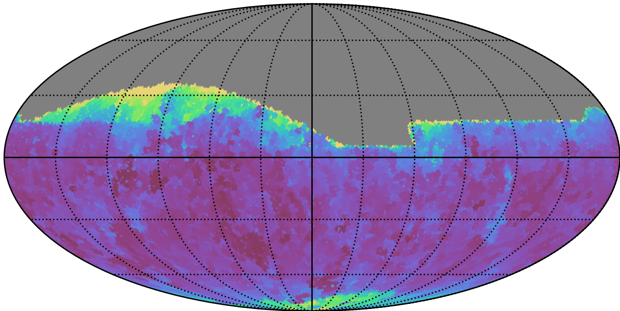
no_high_blob_v3.3_10yrs Yr 1 all bands: Min seeingEff
