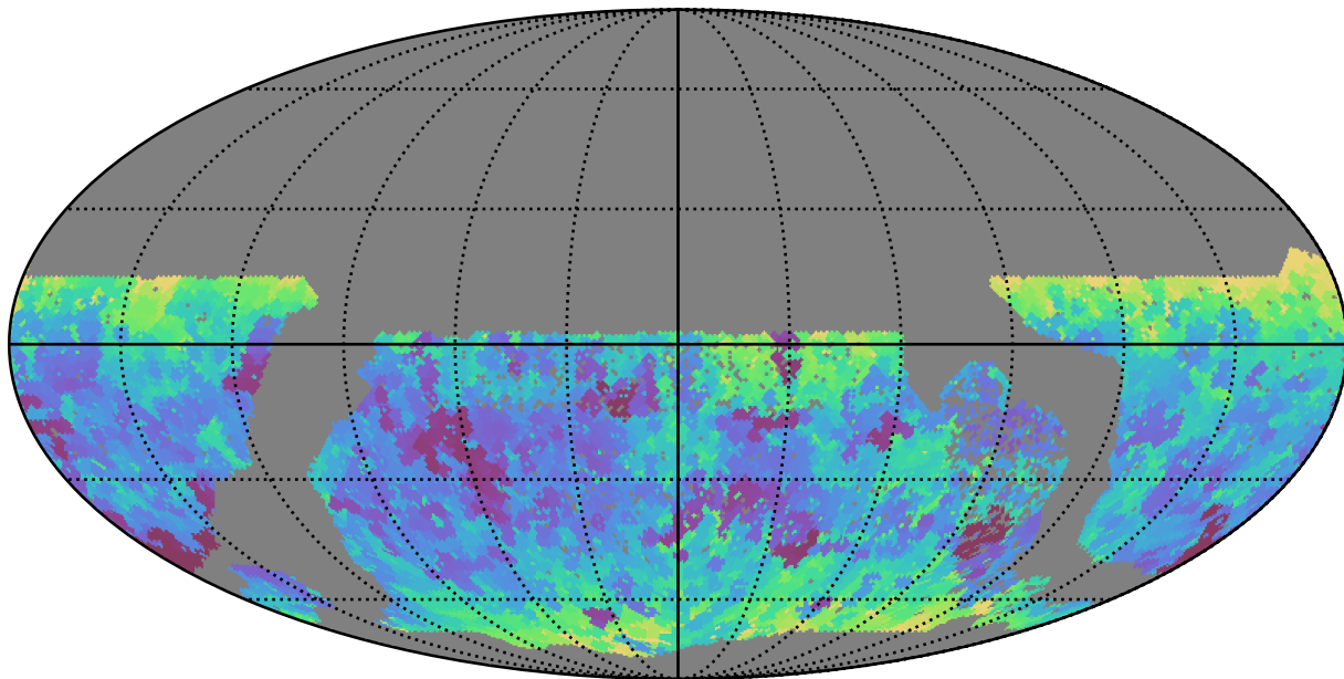
no_high_blob_v3.3_10yrs WFD z band: Min seeingEff
