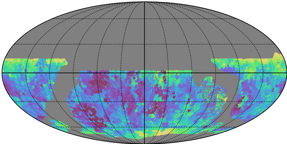
no_high_blob_v3.3_10yrs WFD y band: Min seeingEff
