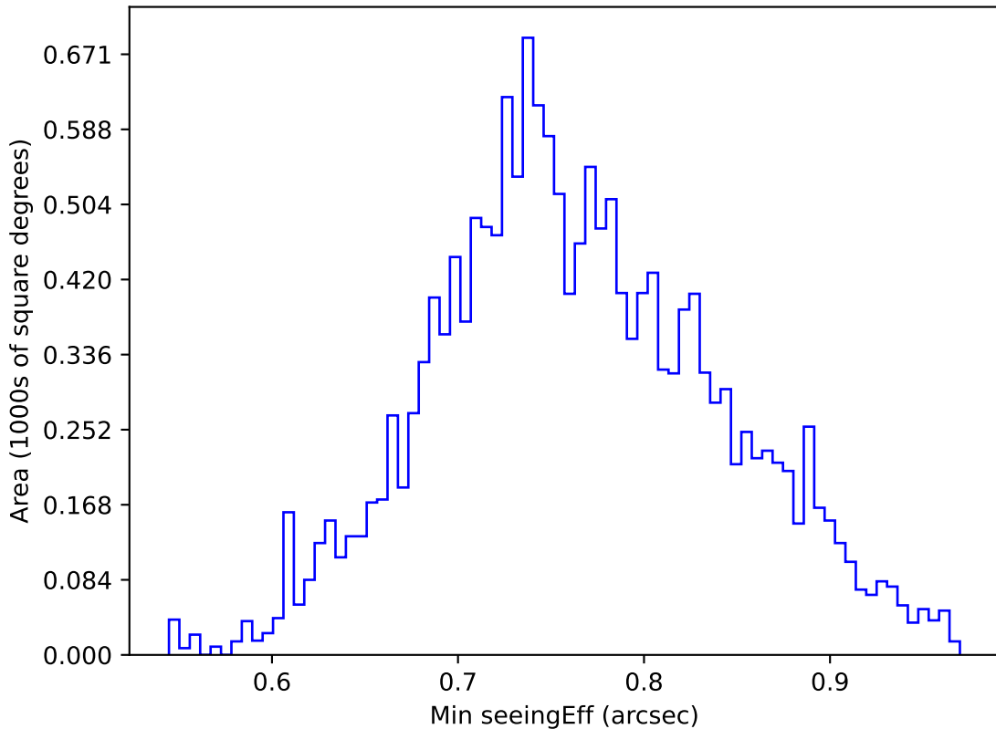
no_high_blob_v3.3_10yrs WFD u band: Min seeingEff
