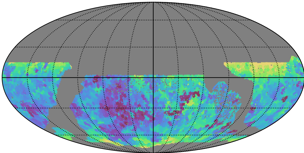
no_high_blob_v3.3_10yrs WFD r band: Min seeingEff
