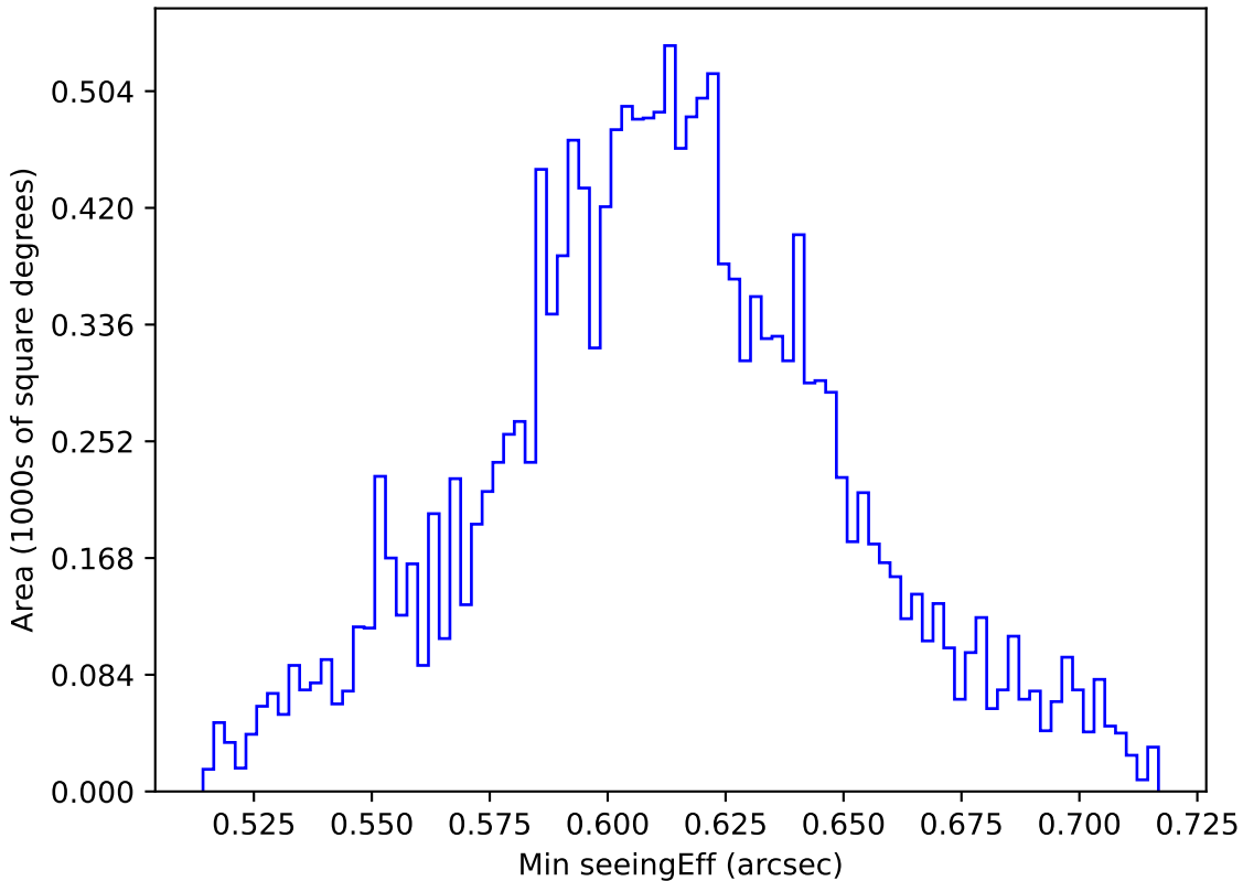
no_high_blob_v3.3_10yrs WFD r band: Min seeingEff
