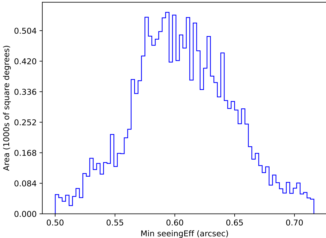
no_high_blob_v3.3_10yrs WFD i band: Min seeingEff
