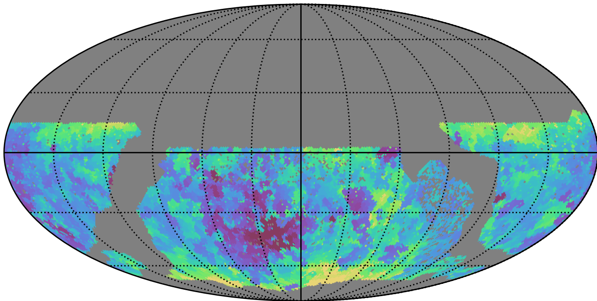
no_high_blob_v3.3_10yrs WFD g band: Min seeingEff
