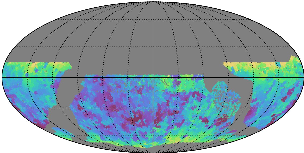
no_high_blob_v3.3_10yrs WFD all bands: Min seeingEff
