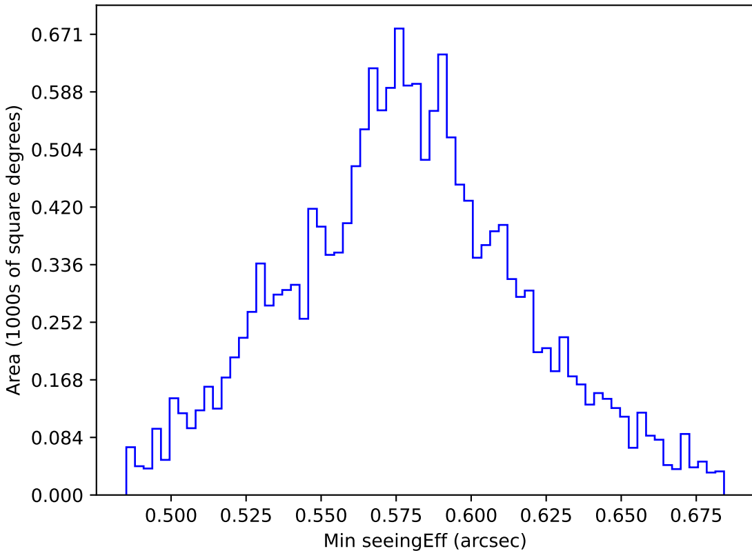
no_high_blob_v3.3_10yrs WFD all bands: Min seeingEff
