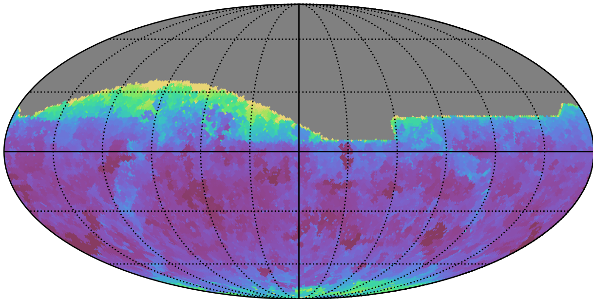
no_high_blob_v3.3_10yrs All sky z band: Min seeingEff
