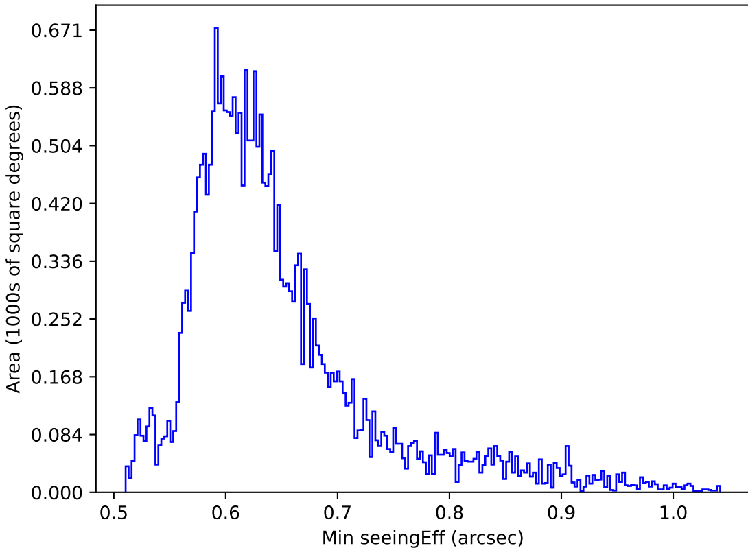
no_high_blob_v3.3_10yrs All sky z band: Min seeingEff
