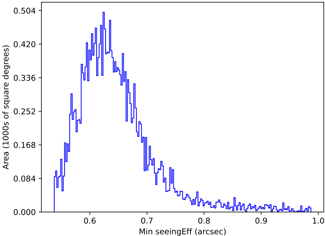
no_high_blob_v3.3_10yrs All sky y band: Min seeingEff
