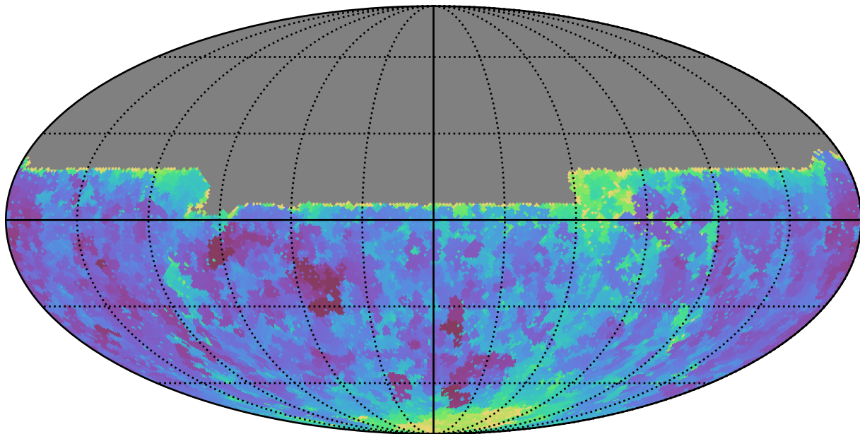
no_high_blob_v3.3_10yrs All sky u band: Min seeingEff
