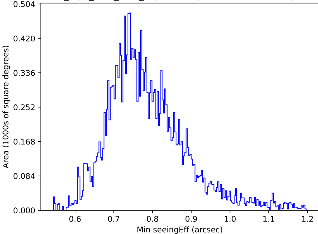
no_high_blob_v3.3_10yrs All sky u band: Min seeingEff
