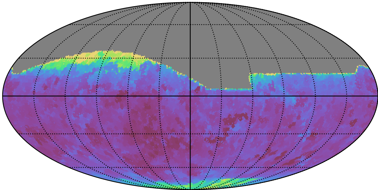
no_high_blob_v3.3_10yrs All sky r band: Min seeingEff
